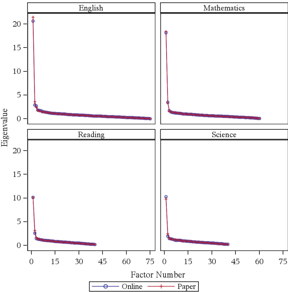
Figure 38. Eigenvalue scree plot for spring 2015
