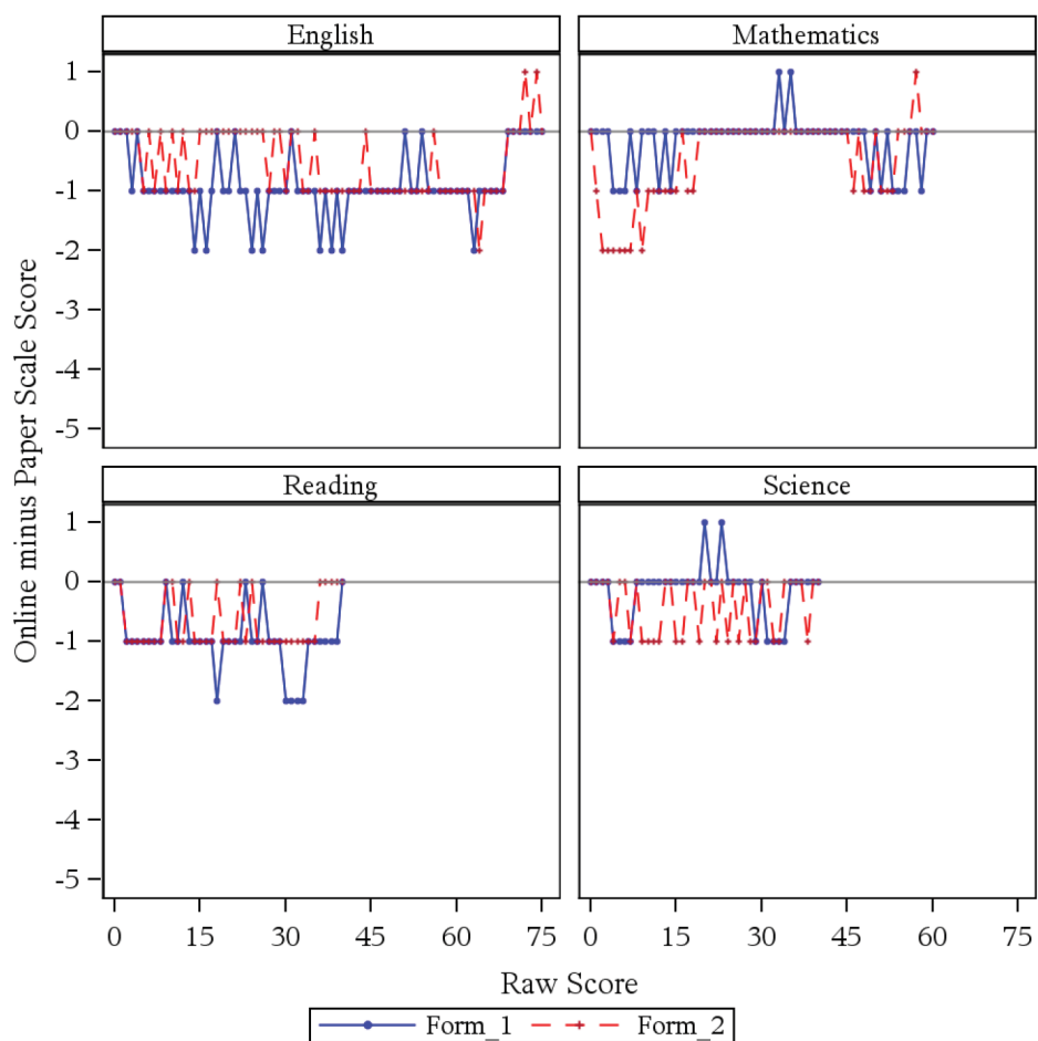
Figure 30. Scale score differences for spring 2015
