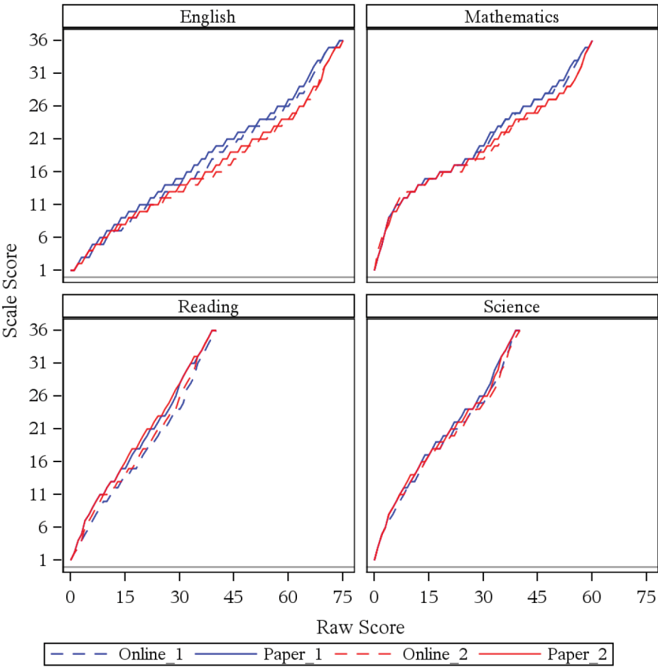
Figure 10. Raw to scale score conversions for spring 2014
