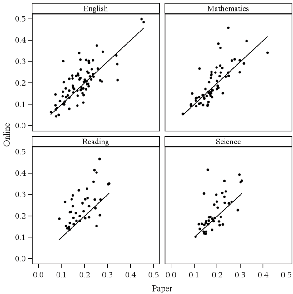
Figure 18. IRT c-parameter comparison across modes for spring 2014
