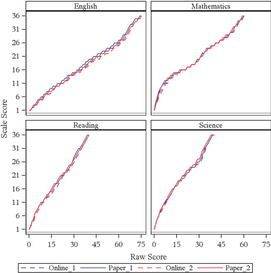
Figure 29. Raw to scale score conversions for spring 2015
