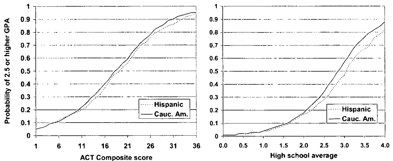
FIGURE 3. Median Within-Racial/Ethnic Group Probabilities of 2.5 or Higher First-Year GPA, Using ACT Composite Score or High School Average (Caucasian-American and Hispanic Students)
