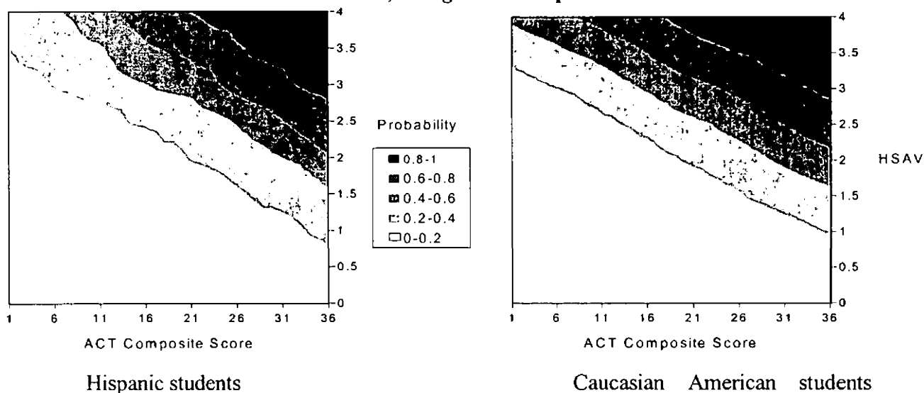
FIGURE 4. Median Within-Group Probabilities of 2.5 or Higher First-Year GPA, Using ACT Composite Score and HSAV
