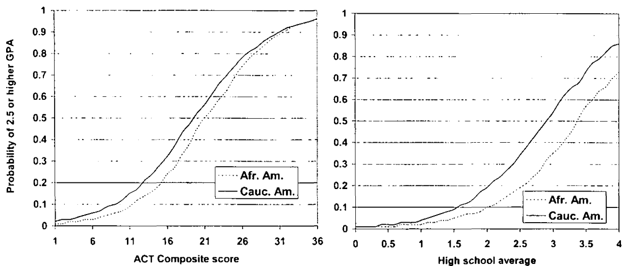
FIGURE 1. Median Within-Racial/Ethnic Group Probabilities of 2.5 or Higher First-Year GPA, Using ACT Composite Score or HSAV (Caucasian American and African American Students)
