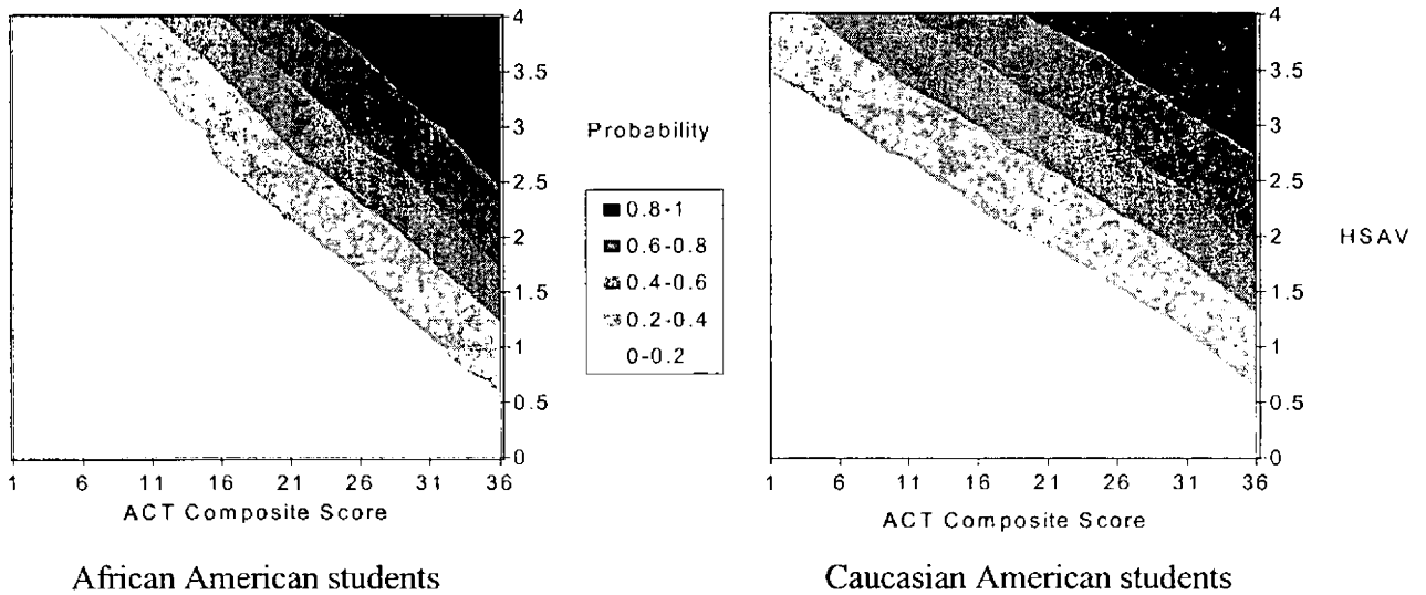
FIGURE 2. Median Within-Group Probabilities of 2.5 or Higher First-Year GPA, Using ACT Composite Score and HSAV
